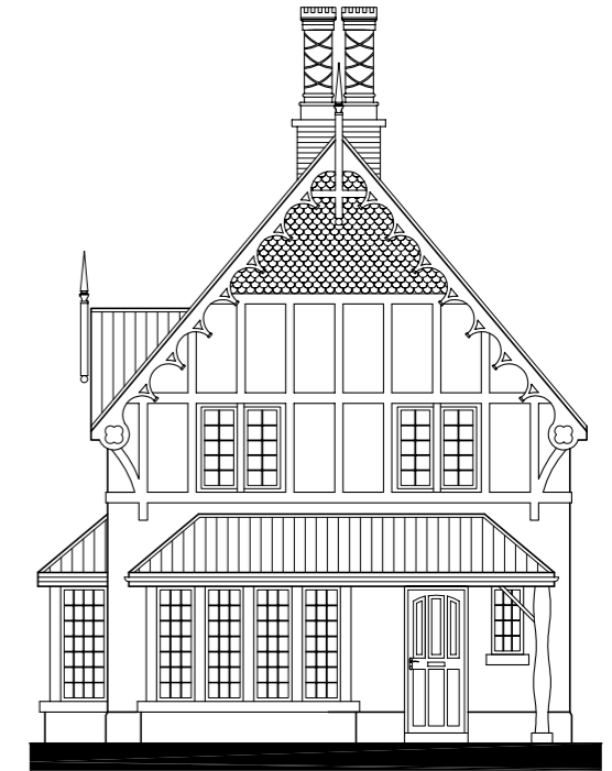
Front Elevation 1/100
