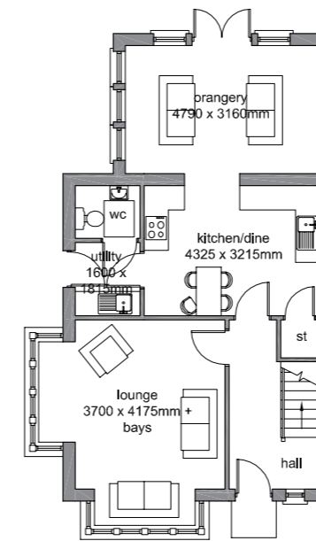
Ground Floor Plan 1/200 1119 sqft
